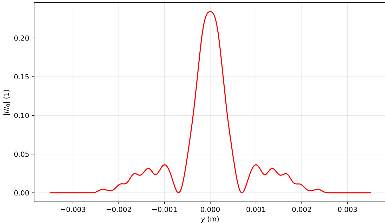
Intensity profile I(x=0, y, z=3.582)/I_0 , P_{in}=8.0P_{cr} , artificial time
